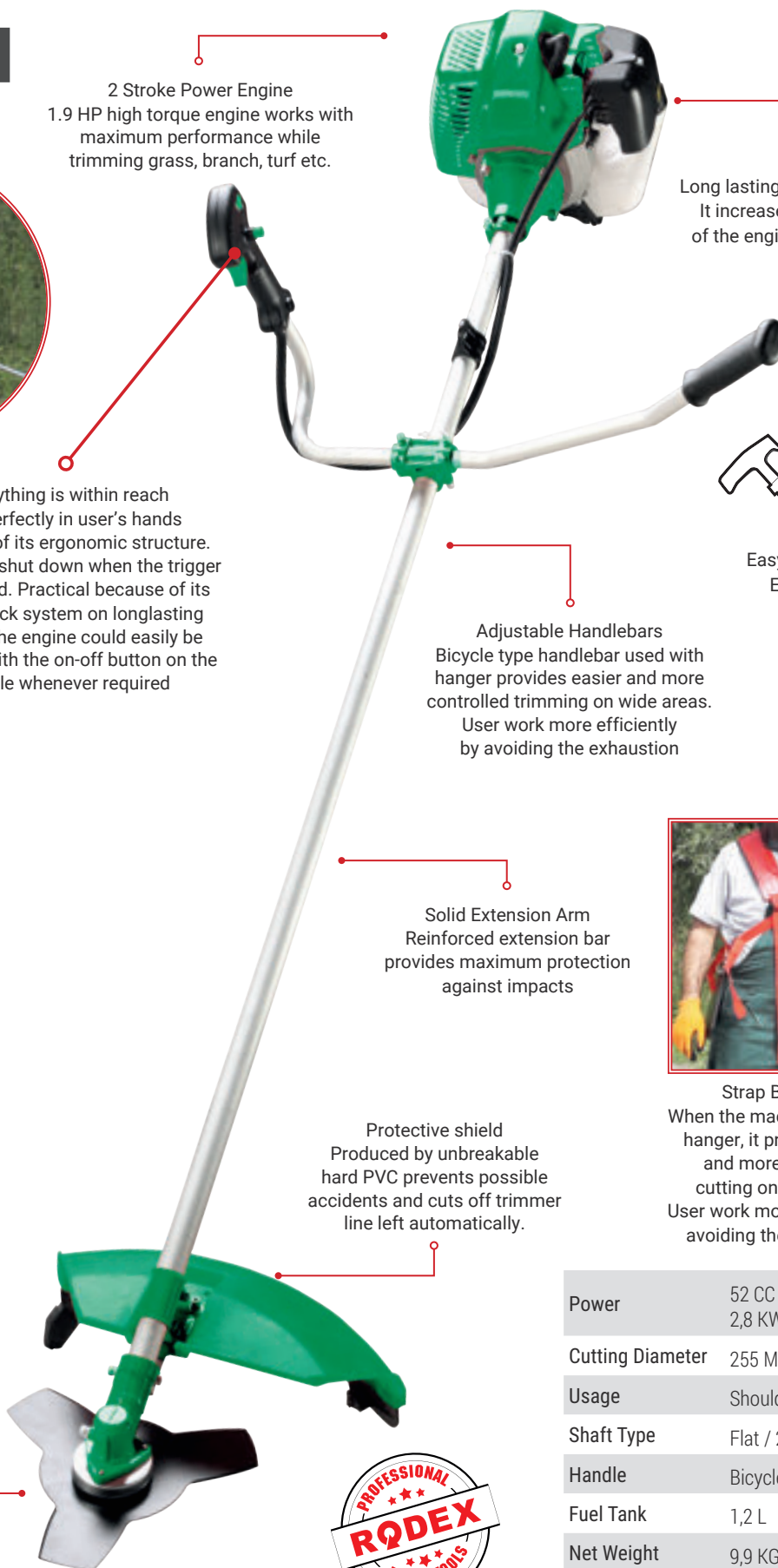
Trimmer Saw
